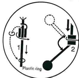
Fig.8: Peel the plastic ring off the counterweight before installation and set them around the cable, then insert the cable from the conic part into the counterweight and fix it with moderate pressure at the fixing end.
