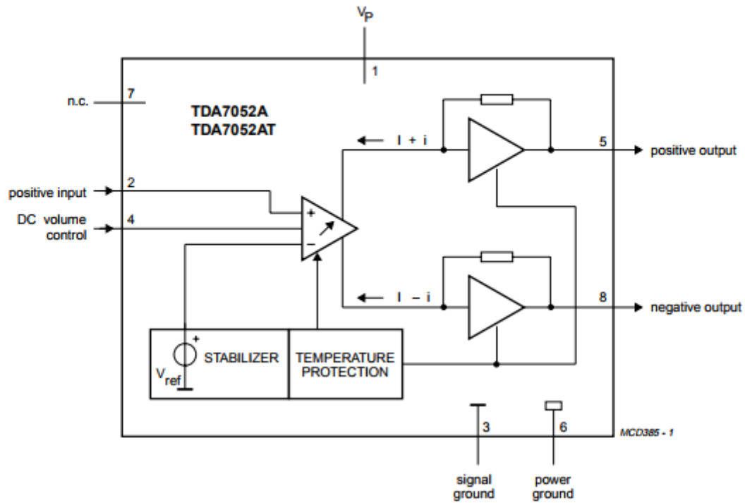
Fig.1 Block diagram.
