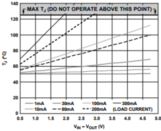
Figure 36. 500 mm 2 of PCB Copper, T_A = 50^\circ\text{C}
