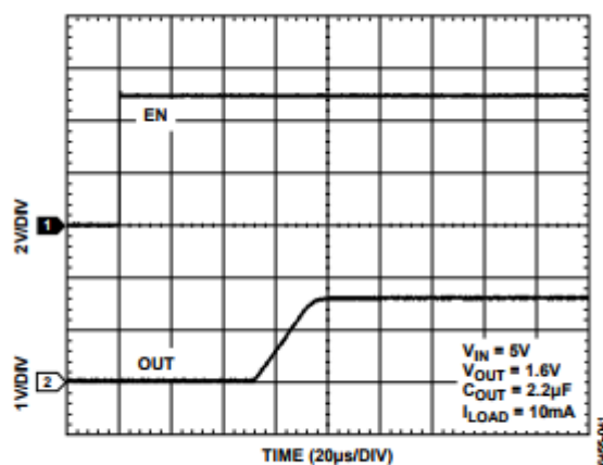
Figure 27. OUT Ramp-Up with Internal Soft-Start
