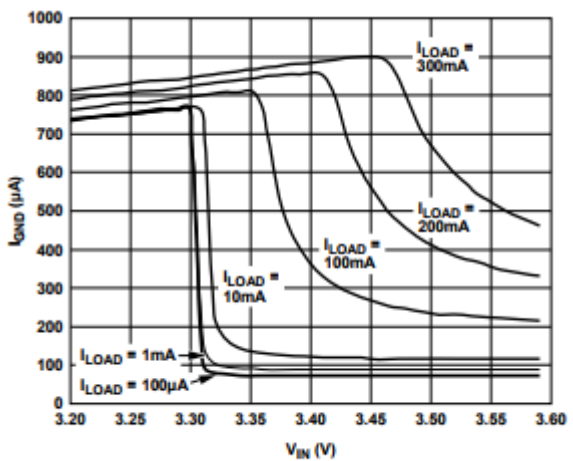
Figure 17. Ground Current vs. Input Voltage (in Dropout)
