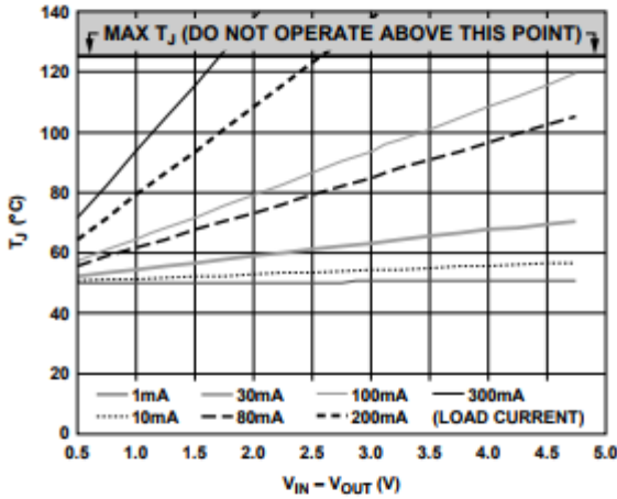
Figure 37. 100 mm 2 of PCB Copper, T_A = 50^\circ\text{C}
