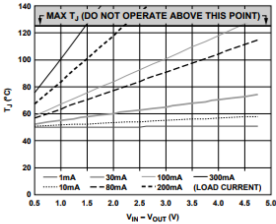
Figure 38. 0 mm 2 of PCB Copper, T_A = 50^\circ\text{C}
