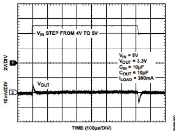
Figure 20. Line Transient Response
