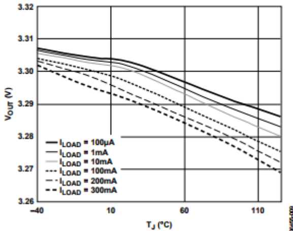
Figure 9. Output Voltage vs. Junction Temperature
