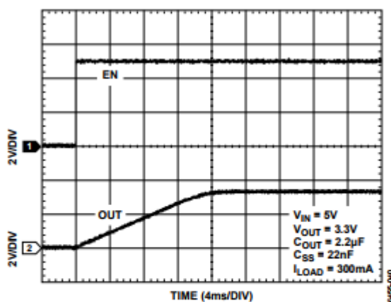
Figure 26. OUT Ramp-Up with External Soft-Start Capacitor
