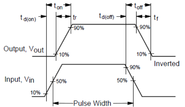
Figure 12. Switching Waveforms.
