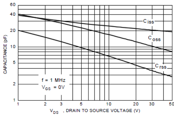
Figure 9. Capacitance Characteristics.
