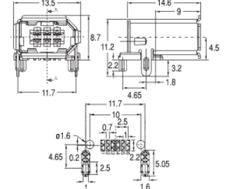
IEEE 1394 (SMD)
