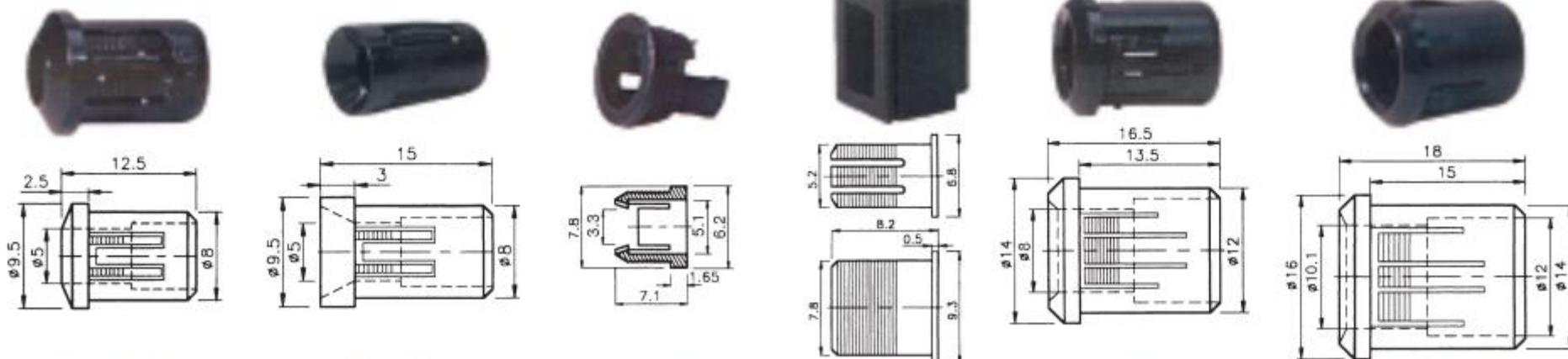
RTF-5010 Ø5 mm
