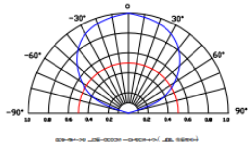
Radiation pattern.
