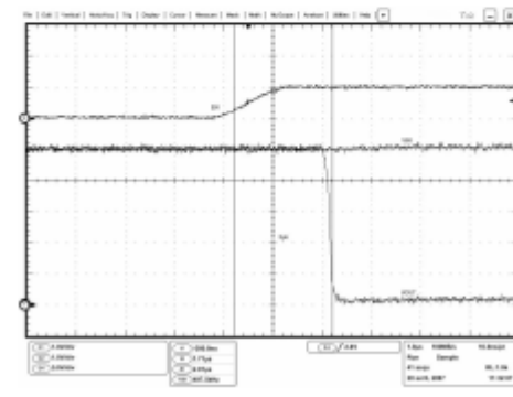
Figure 13. Disable Time. EN=Ch4, Vin=Ch1, Vout=Ch2
