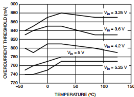
Figure 18. Overcurrent Protection Threshold vs. Temperature
