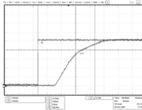
Figure 9. Start Up. Vin=Ch1, Vout=Ch2
