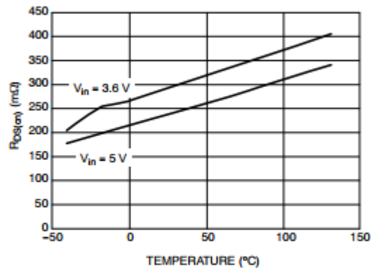
Figure 15. R_{DS(on)} vs. Temperature (Load = 500 mA)
