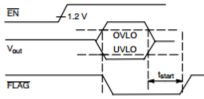
Figure 6. FLAG Response with EN = 1
