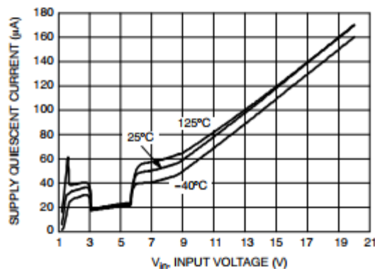
Figure 17. Quiescent Current vs. Input Voltage
