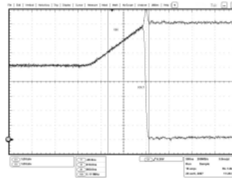
Figure 11. Output Turn Off time. Vin=Ch1, Vout=Ch2
