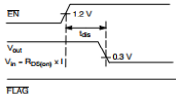
Figure 5. Disable on EN = 1
