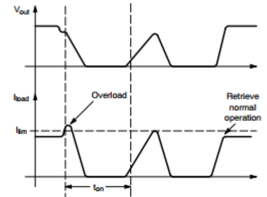
Figure 21. Overcurrent Event Example
