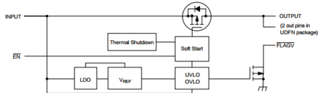
Figure 2. Functional Block Diagram
