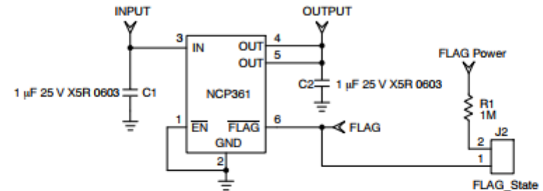
Figure 1. Typical Application Circuit (UDFN Pinout)
