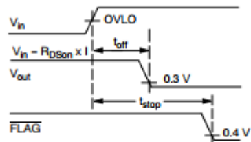
Figure 4. Shutdown on Over Voltage Detection
