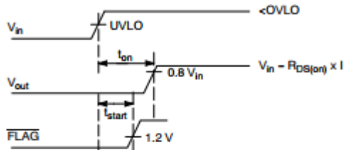
Figure 3. Start Up Sequence
