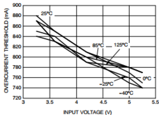
Figure 19. Overcurrent Protection Threshold vs. Input Voltage
