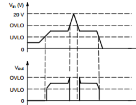
Figure 20. Output Characteristic vs. V_{in}
