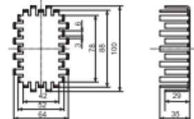
203 64x100x35 mm
