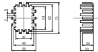
202 56x72x30 mm
