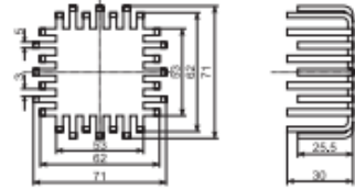
105 71x71x30 mm
