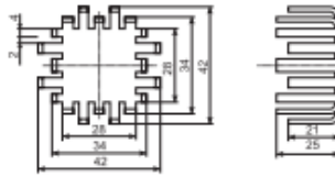
102 42x42x25 mm
