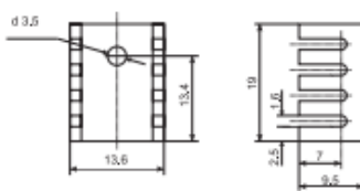
718 19x13.6x9.5 mm
