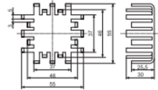
103 55x55x30 mm
