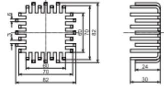
106 82x82x30 mm
