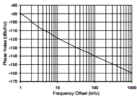
ROS-369-319+ Phase Noise
