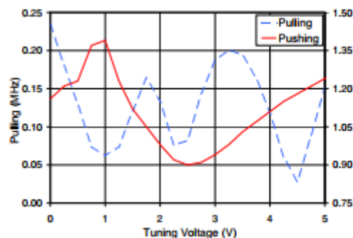
ROS-369-319+ Frequency Pulling & Pushing (Vcc ± 5%)
