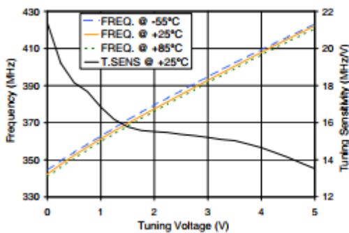
ROS-369-319+ Frequency and Tuning Sensitivity
