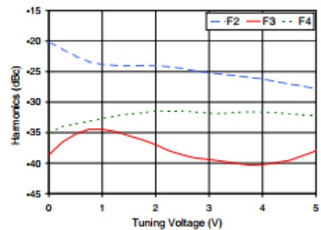
ROS-369-319+ Harmonics Level
