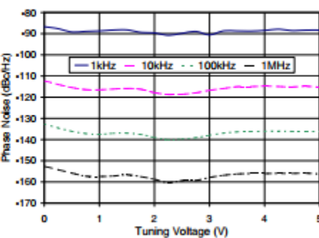
ROS-369-319+ Phase Noise Vs. Tuning Voltage
