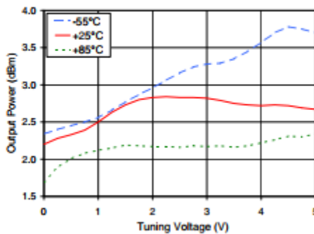
ROS-369-319+ Power Output
