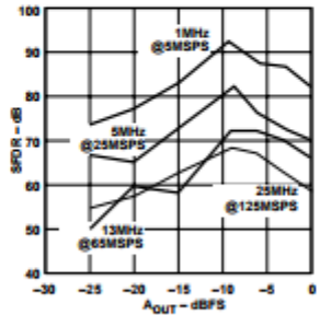
Figure 10. Single-Tone SFDR vs. A_{OUT} @ f_{OUT} = f_{CLOCK}/5
