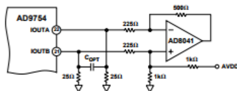
Figure 29. Single-Supply DC Differential Coupled Circuit
