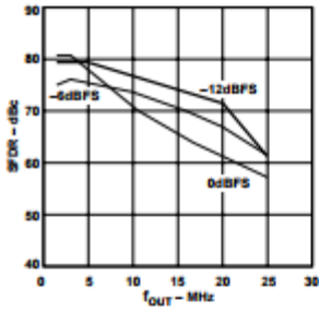
Figure 6. SFDR vs. f_{OUT} @ 65 MS/PS
