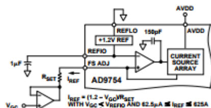
Figure 20. Dual-Supply Gain Control Circuit
