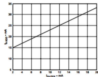
Figure 24. I AVDD vs. I OUTFS
