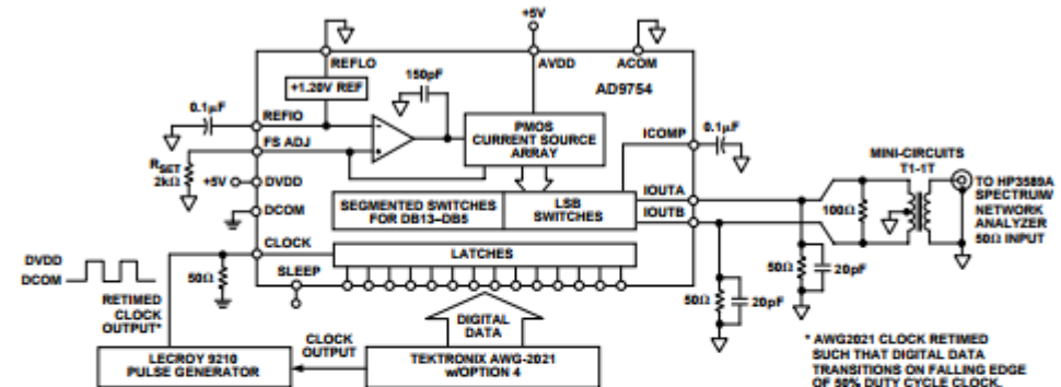
Figure 2. Basic AC Characterization Test Setup
