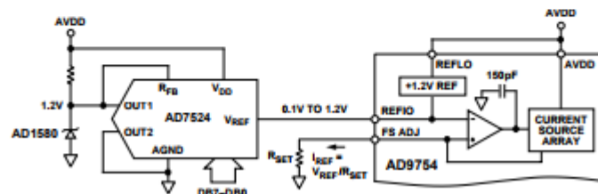
Figure 19. Single-Supply Gain Control Circuit
