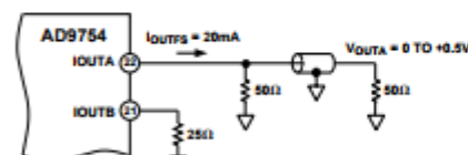
Figure 30. 0 V to +0.5 V Unbuffered Voltage Output
