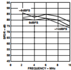
Figure 5. SFDR vs. f_{OUT} @ 25 MS/PS
