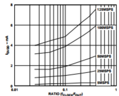
Figure 26. I DVDD vs. Ratio @ DVDD = 3 V
