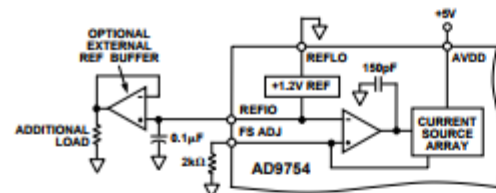
Figure 17. Internal Reference Configuration
