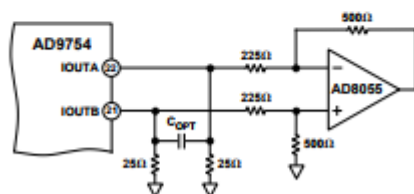
Figure 28. DC Differential Coupling Using an Op Amp
