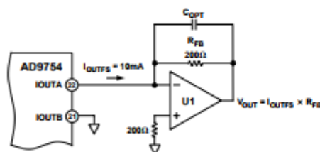
Figure 31. Unipolar Buffered Voltage Output
