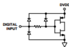
Figure 22. Equivalent Digital Input
