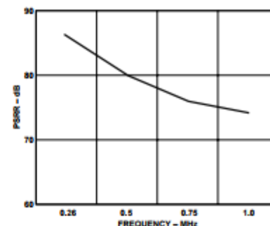
Figure 32. Power Supply Rejection Ratio of AD9754
