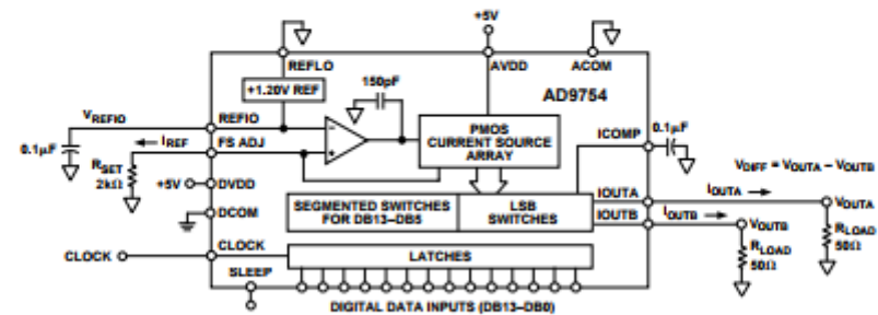
Figure 16. Functional Block Diagram
