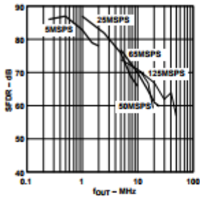
Figure 3. SFDR vs. f_{OUT} @ 0 dBFS
