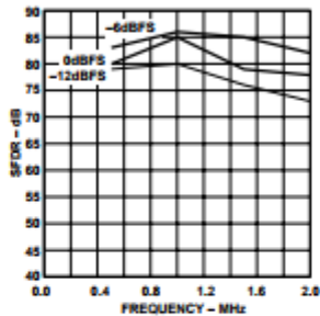
Figure 4. SFDR vs. f_{OUT} @ 5 MS/PS
