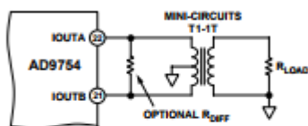
Figure 27. Differential Output Using a Transformer
