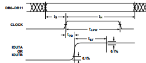
Figure 1. Timing Diagram
