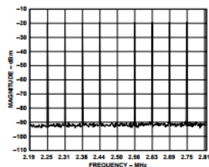
Figure 34a. Multitone Spectral Plot
