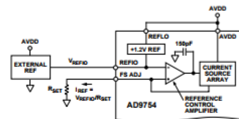
Figure 18. External Reference Configuration
