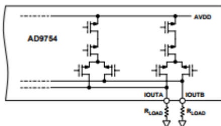
Figure 21. Equivalent Analog Output Circuit
