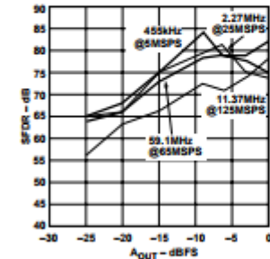
Figure 9. Single-Tone SFDR vs. A_{OUT} @ f_{OUT} = f_{CLOCK}/11
