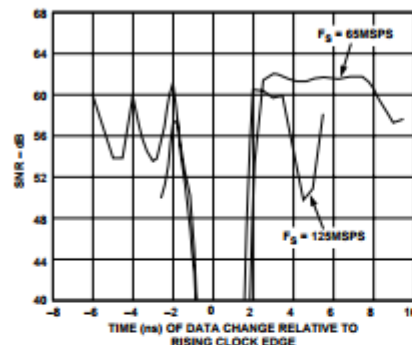
Figure 23. SNR vs. Clock Placement @ f OUT = 10 MHz
