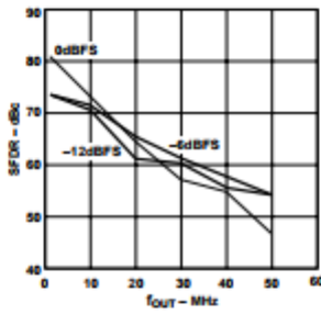
Figure 7. SFDR vs. f_{OUT} @ 125 MS/PS
