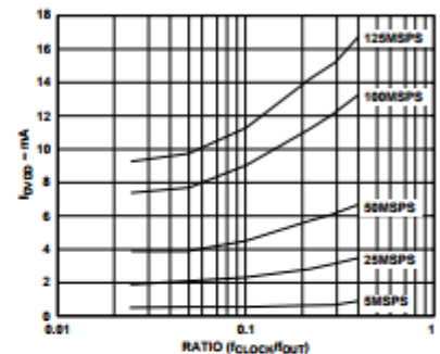
Figure 25. I DVDD vs. Ratio @ DVDD = 5 V
