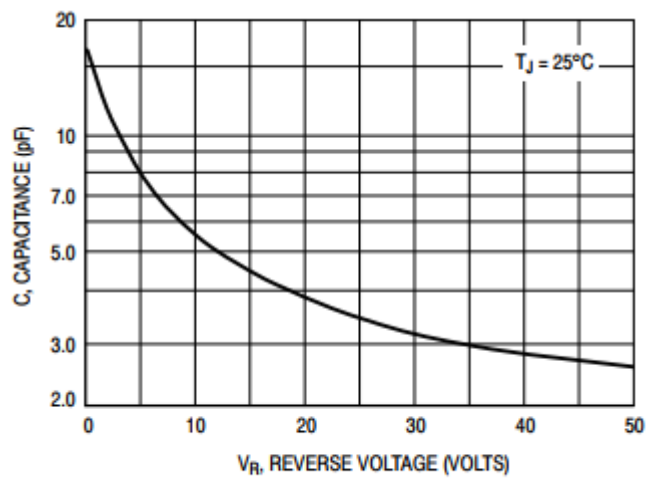
Figure 5. Typical Capacitance
