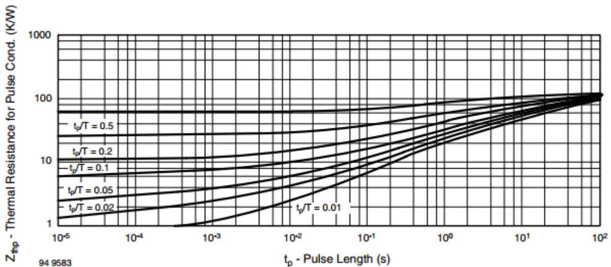
Fig. 5 - Thermal Response
