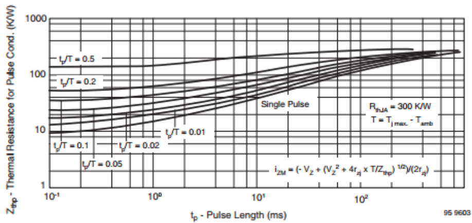
Fig. 10 - Thermal Response
