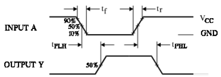
Figure 1. Switching Waveforms
