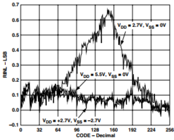
TPC 3. AD5200 10 kΩ RINL vs. Code
