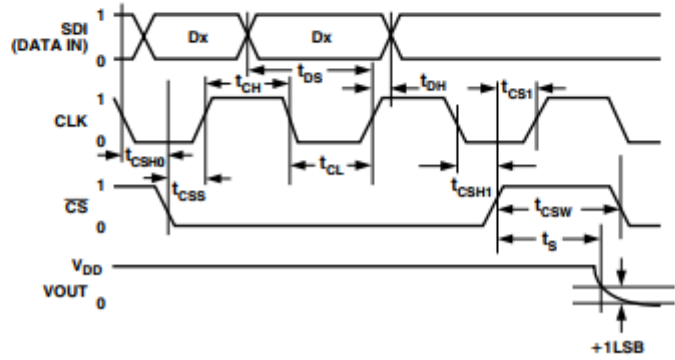
Figure 1c. Detail Timing Diagram
