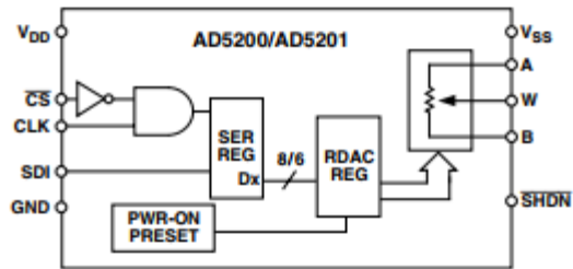
Figure 3. Block Diagram
