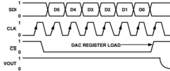
Figure 1b. AD5201 Timing Diagram
