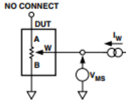
Figure 7. Resistor Position Nonlinearity Error (Rheostat Operation; R-INL, R-DNL)
