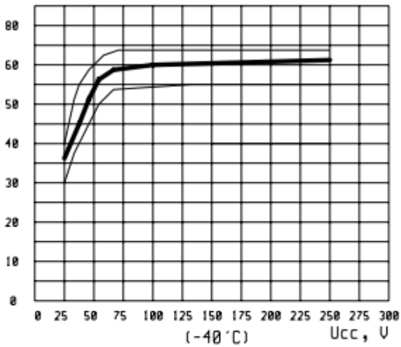
I_{del}(ON) , \mu A
