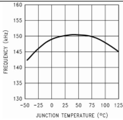
Figure 11. Switching Frequency
