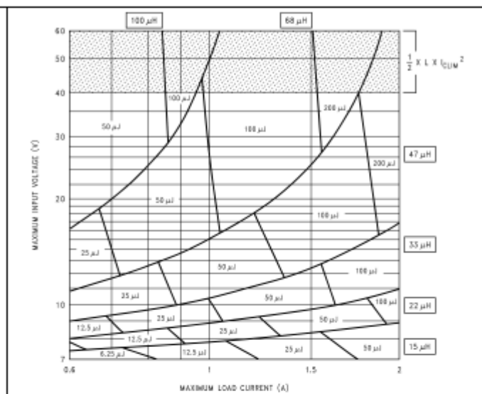
Figure 29. LM2592HV-5.0
