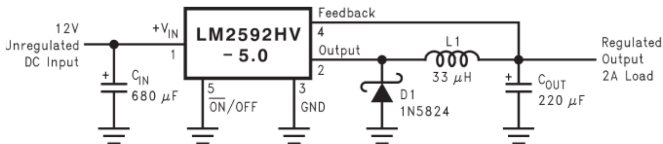
Figure 27. Typical Application
