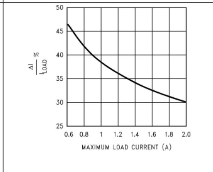
Figure 31. Current Ripple Ratio
