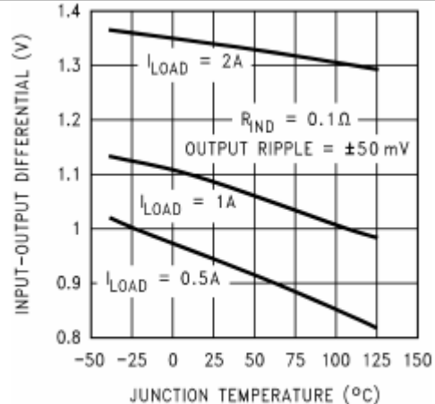
Figure 6. Dropout Voltage
