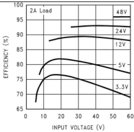
Figure 3. Efficiency
