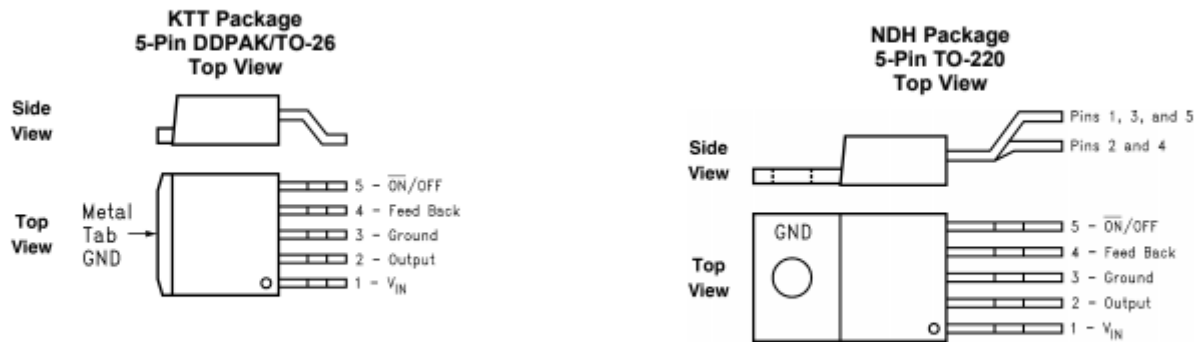
Pin Functions
