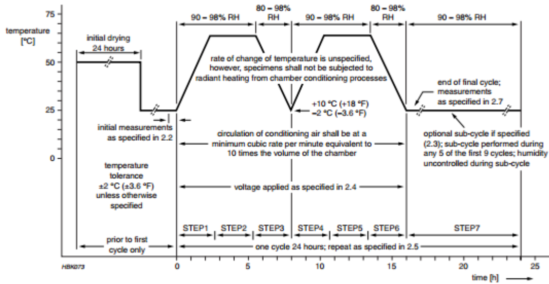
Fig. 6 Moisture resistance test requirements
